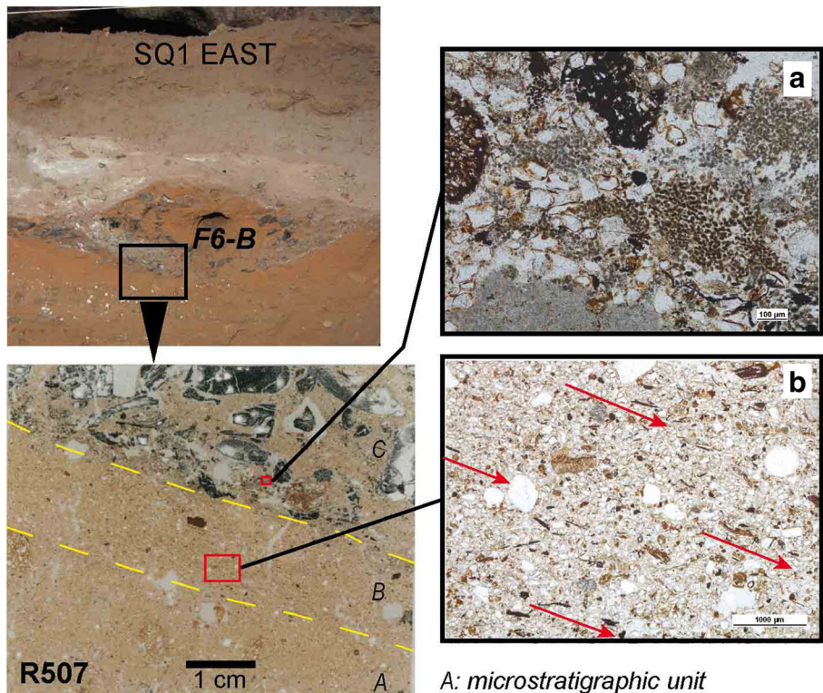
Fig. 8 Microfacies types in Pleistocene type B dug combustion features (modified from Vannieuwenhuysen 2016). Top left, detailed view of combustion feature F6-B in Riwi square 1 east section showing location of micromorphological sample. Bottom left, scan of thin section R507 showing the different microstratigraphic units identified. Right, microphotographs of two different microfacies identified. a Mixed charcoal fragments, ash particles and geogenic sands (R507C, PPL, scale 100 µm); b bedded organic particles below the combustion feature that could indicate digging, the particles being oriented in the same direction due to sloping (R507A, PPL, scale 1000 µm)
