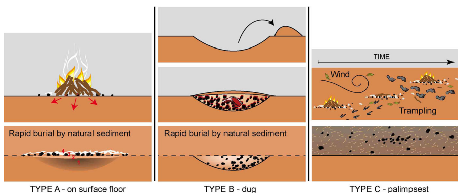
Fig. 4 Combustion feature types found in Riwi (modified from Vannieuwenhuysen 2016)
