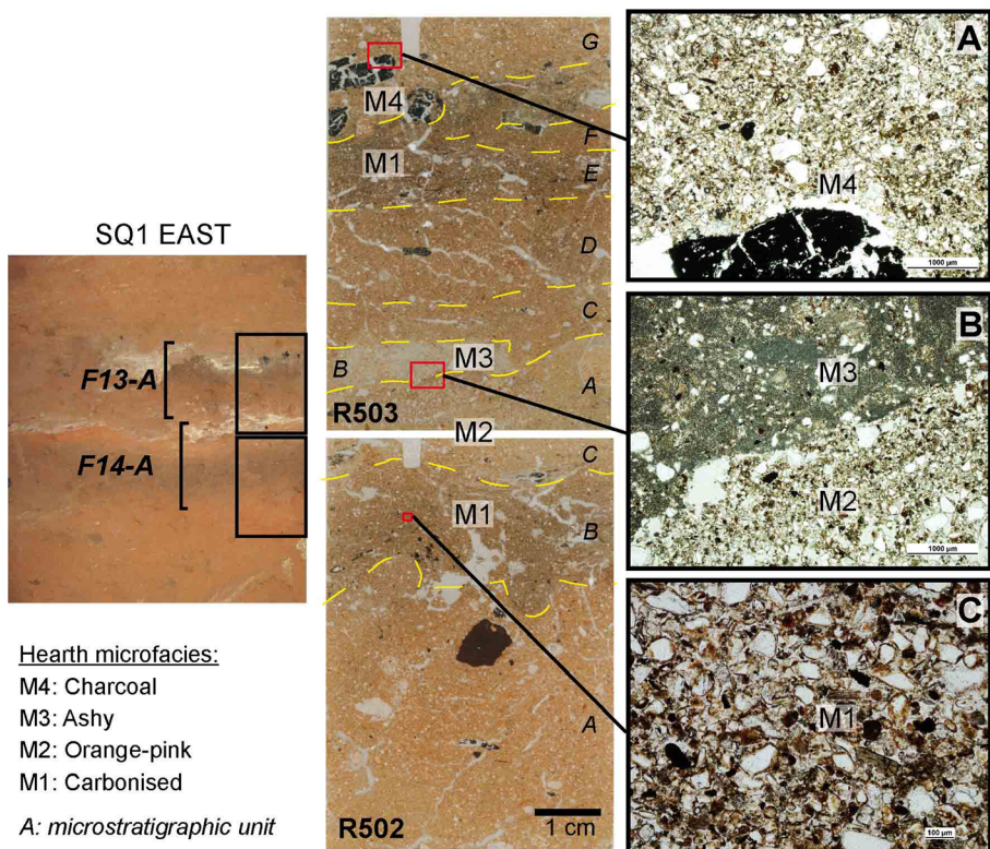
Fig. 7 Microfacies types in Pleistocene type A flat combustion features (modified from Vannieuwenhuyse 2016). Left, detailed view of flat combustion features F13-A and F14-A in Riwi square 1 eastern section showing location of micromorphological samples. Middle, scan of thin sections R502 and R503 with microstratigraphic units identified in each thin section, microphotos location and hearth microfacies types (M1 to M4). Right, microphotographs of type A flat combustion features microfacies types (numbering in reference to Fig. 4 and in-text description). a Top layer with charcoal fragments (microfacies 3) (F13-A, R503G, PPL, scale 1000 µm); b orange-pinkish (microfacies 2) and whitish layers (microfacies 4) (F14-A, R503A/B, PPL, scale 1000 µm); c dark carbonised organic-rich layer (microfacies 1) (F14-A, R502B, PPL, scale 100 µm)
